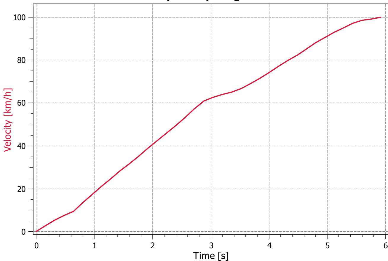
Speed-up diagram
